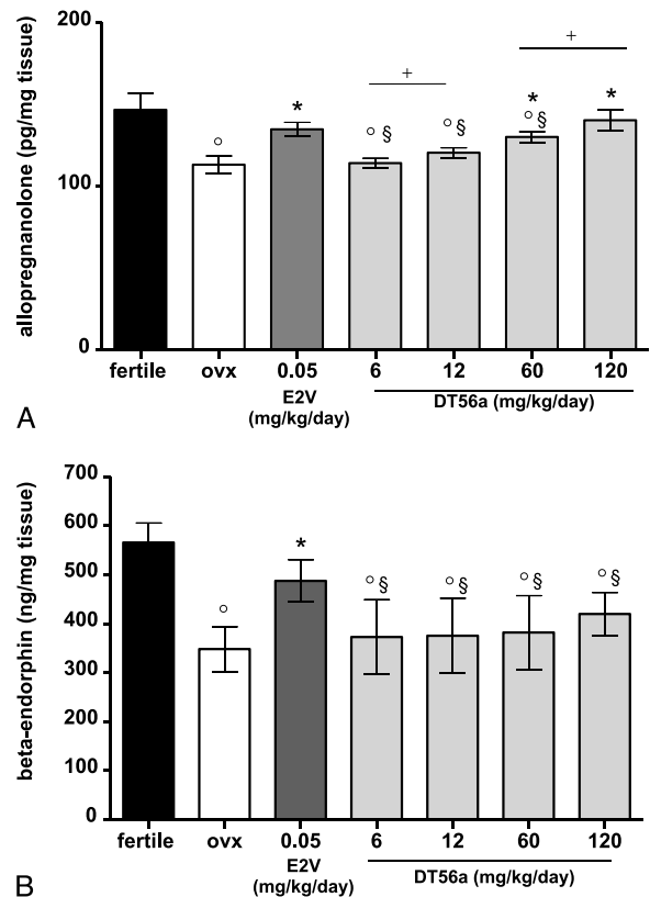
FIG. 1. Allopregnanolone (A) and \beta -endorphin (B) levels in frontal cortex of seven groups of eight animals each. Fertile, fertile rats; OVX, ovariectomized rats; E2V, estradiol valerate. ° , vs fertile ( ° P < 0.05); *, vs OVX (* P < 0.05); +, vs other treatment dose (+ P < 0.05); §, vs E2V (§ P < 0.05).
